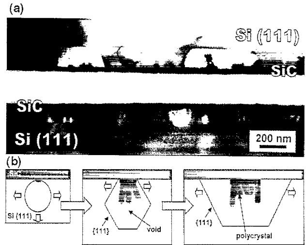
Fig. 5. (a) Low magnification bright field cross-sectional transmission electron microscopy image on a \{110\} projection showing a general view of the SiC layer and faceted and non-faceted voids in the \{111\} Si substrate. (b) Scheme of the void growth.
