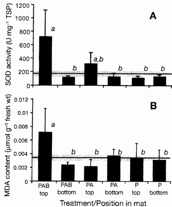
Fig. 5. Chaetomorpha linum . (A) Activity of superoxide dismutase (SOD), expressed as units mg -1 total soluble protein (TSP), and (B) degree of lipid peroxidation, measured as formation of malondialdehyde (MDA), in top and bottom layers of artificial mats exposed to solar PAR + UV-A + UV-B (PAB), PAR + UV-A (PA) or PAR (P) sampled at 14:00 h on 5 September (n = 3). Values are means (+SD). Black horizontal line shows mean of initial samples taken from subcanopy (grey horizontal shading = SD). Different letters above bars indicate significantly different values (p < 0.05) determined by post-hoc comparison
