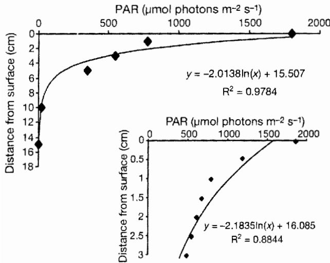
Fig. 2. Gradient of photosynthetically active radiation (PAR) within natural mats of Chaetomorpha linum measured by the light sensor of an underwater chlorophyll fluorometer (Diving-PAM) previously intercalibrated with Licor sensors. Inset: light gradient in artificial algal mats
