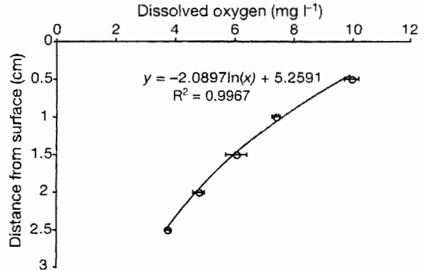
Fig. 3. Chaetomorpha linum . Typical gradient of dissolved oxygen in artificial mats measured by microelectrodes. Example is for mats under PAR + UV-A treatment on 5 September at 14:00 h. Note: oxygen content shown is product of photosynthesis and respiration within thallus fragments, but is also affected by water motion and diffusion
