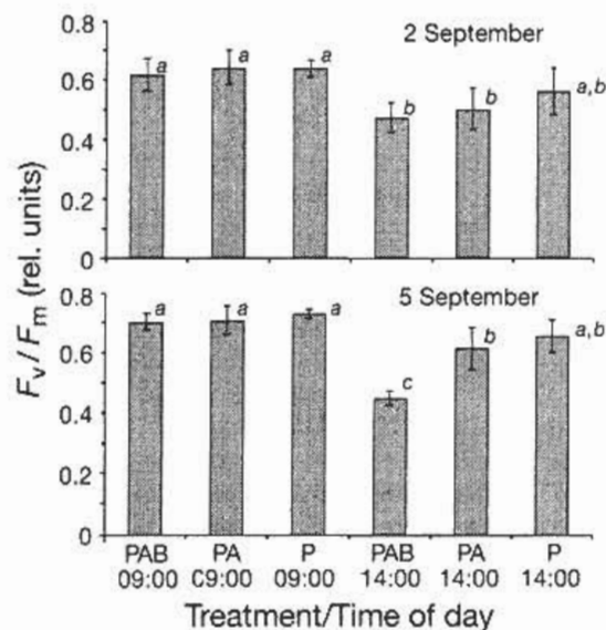
Fig. 4. Chaetomorpha linum . Mean (+SD) differences in maximal quantum yield of photosynthesis ( F_v/F_m ) in surface layers of artificial mats exposed to solar PAR + UV-A + UV-B (PAB), PAR + UV-A (PA) or PAR (P) alone, measured in morning (09:00 h) and afternoon (14:00 h) of 2 and 5 September ( n = 5). Different letters above bars indicate significantly different values ( p < 0.05) determined by post-hoc comparison
