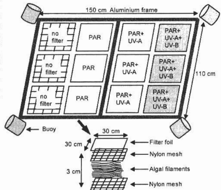
Fig. 1. Floating experimental set-up consisting of aluminium frames attached to buoys and holding 12 artificial mats of Chaetomorpha linum , either covered with nylon mesh only ('no filter'), or with different filter foils. Filter foils were held in desired position by tie-wraps
