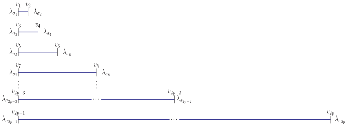
Fig. 2. The new representation of the graph where \sigma_{2i} > \sigma_{2i-1} , for i = 1, \dots, p and \sigma_{2i+2} > \sigma_{2i} , for i = 1, \dots, p - 1 .
