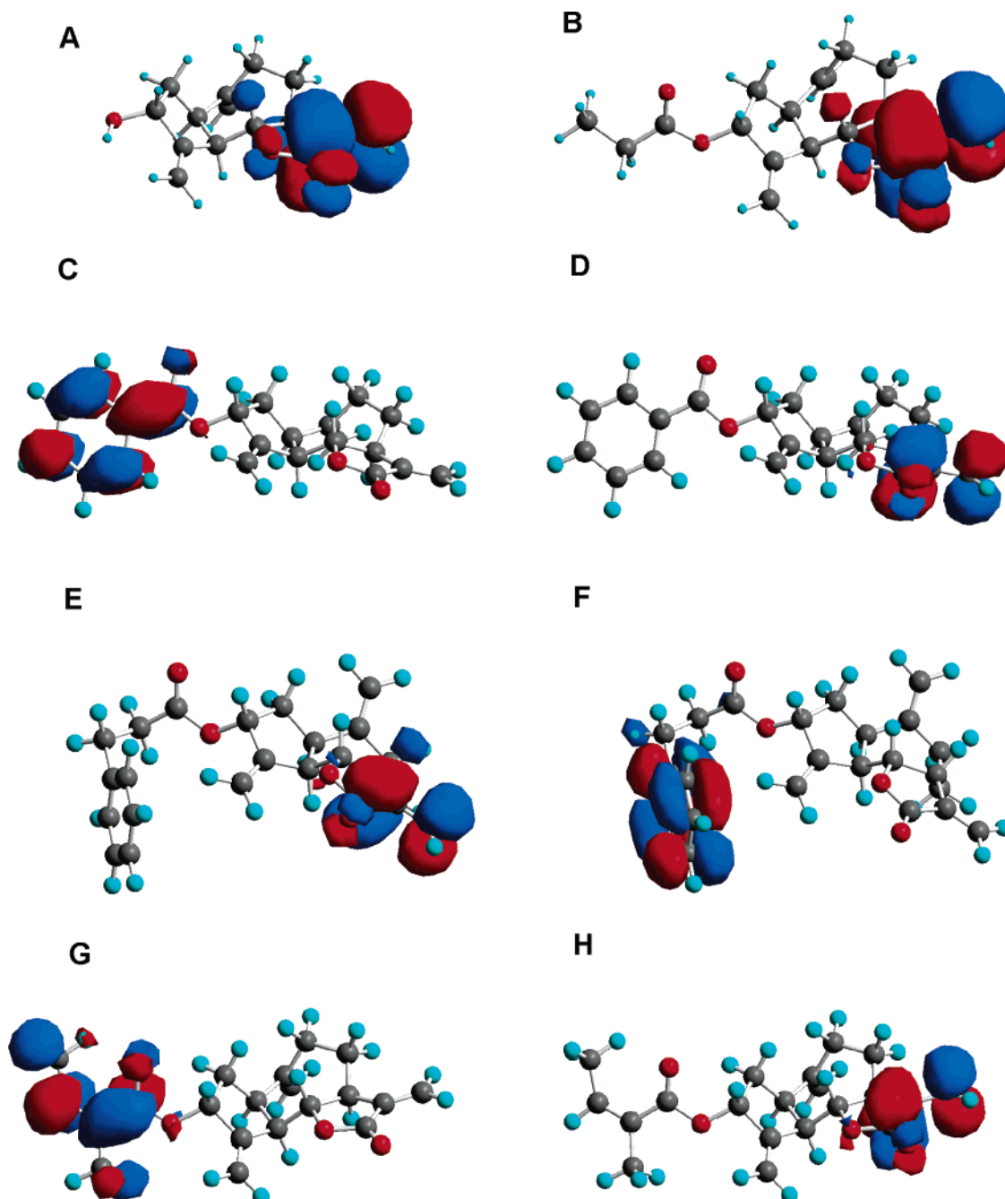
Figure 5. MOs involved in the Michael addition of a bionucleophile to the SL tested. Isozaluzanin C (1): (A) LUMO ( E = -0.224994 eV); propionyloxyisozaluzanin C (3): (B) LUMO ( E = -0.22079 eV); benzoyloxyisozaluzanin (13): (C) LUMO ( E = -0.696346 eV) and (D) LUMO + 1 ( E = -0.196523 eV); dihydrocinnamoyloxyisozaluzanin C (15): (E) LUMO ( E = -0.968833 eV) and (F) LUMO + 1 ( E = -0.233009 eV); tigloyloxyisozaluzanin C (16): (G) LUMO ( E = -0.210318 eV) and (H) LUMO + 1 ( E = -0.198057 eV).
