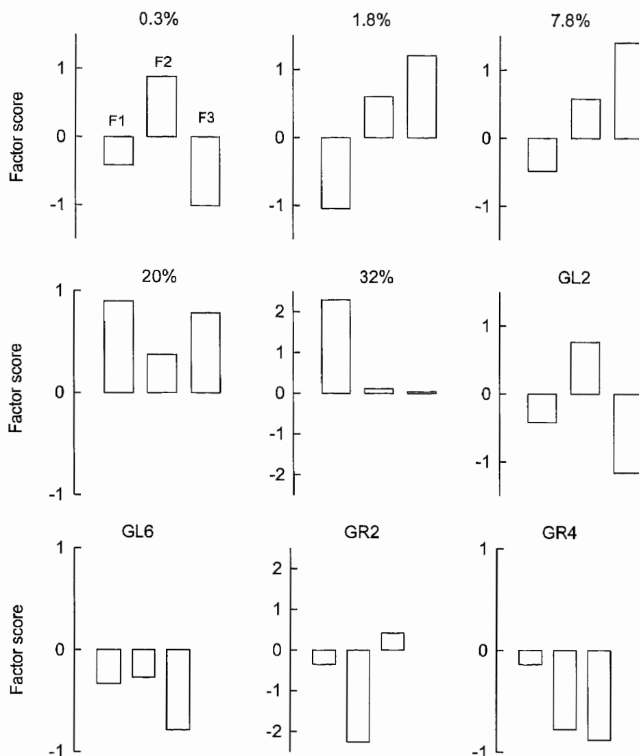
Figure 2. Estimated factor scores for each of the nine cases evaluated using five toxic mud dilutions (0.3%, 1.8%, 7.8%, 20% and 32% dry weight of toxic mud) and sampling points located in the Guadalquivir estuary (GL2, GL6, GR2 and GR4) to the centroid of all cases for the original data. The factor scores quantify the prevalence of every factor for each station and are used to calculate the sediment quality guidelines (SQGs).
