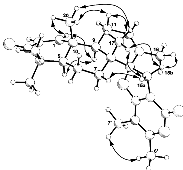
Fig. 3. Observed NOEs for the most stable conformer of 1 using PM3 calculations
