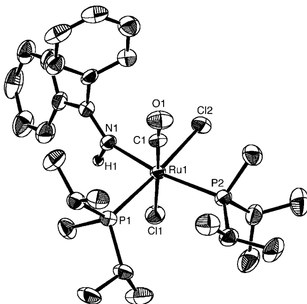
Fig. 1 An ORTEP 15 drawing of the compound [RuCl 2 (CO)(NH=CPh 2 )-(P i Pr 2 Me) 2 ] 4 .
