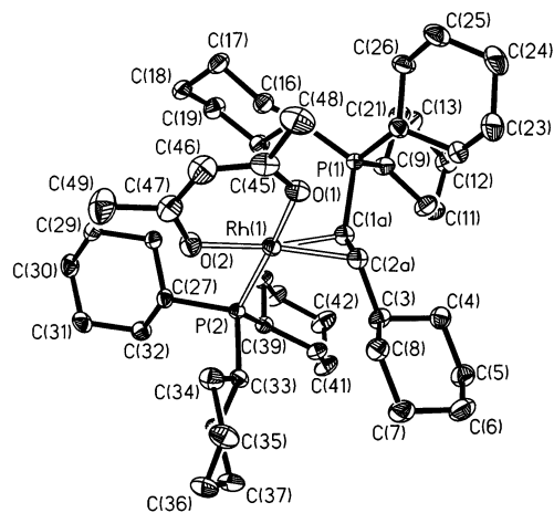
Fig. 1. Molecular representation for the cationic complex [Rh(acac){η 2 -( E )-CH(PCy 3 )=CHCy}(PCy 3 )][BF 4 ] (4). Only one group of atoms has been drawn for the disordered olefinic carbon atoms.
