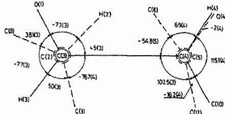
Fig. 3. Newman projections illustrating the coupling of the three fused rings in the molecule. Torsion angles are in ^\circ .
