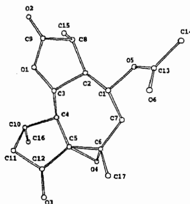
Fig. 1. A view of the molecule in the xy projection.
