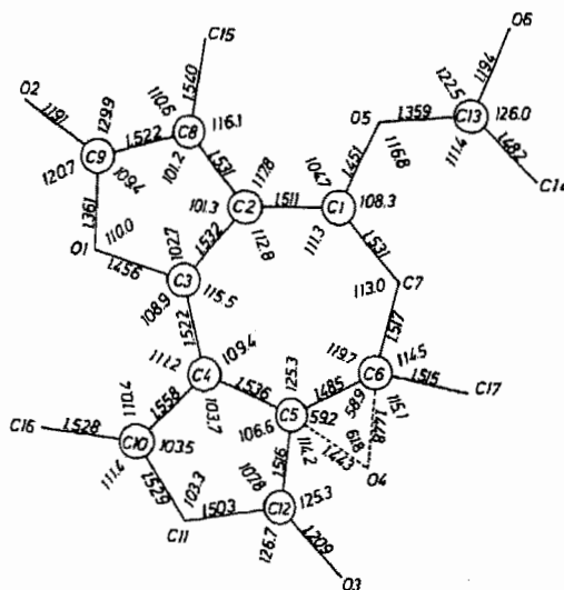
Fig. 2. Bond distances ( \text{\AA} ) and angles ( ^\circ ) in the molecule. Values of angles C(6)-C(5)-C(12), C(5)-C(6)-C(17), O(4)-C(5)-C(4) and O(4)-C(6)-C(7) are 123.8 (3), 122.1 (3), 119.8 (3) and 113.4 (3) ^\circ , respectively. Standard deviations are in the ranges 0.004-0.007 \text{\AA} for distances and 0.3-0.4 ^\circ for angles.
