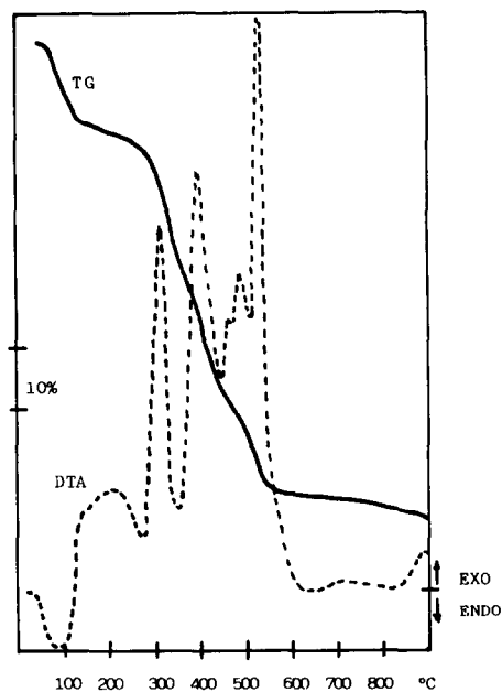
Fig. 2. DTA and TG curves for \text{Na}[\text{Cr}(\text{CDTA})\text{N}_2]\cdot 2\text{H}_2\text{O} .
