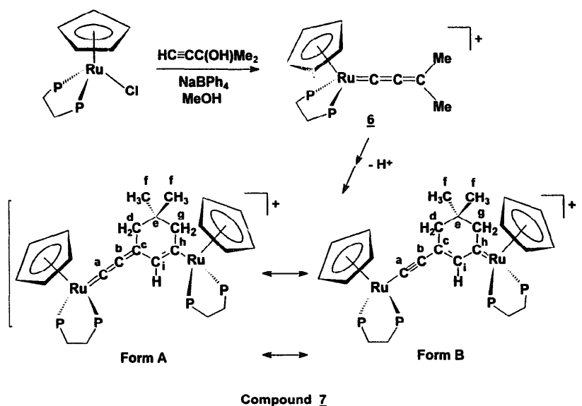
Scheme 1. Interaction of [\text{CpRuCl}(\text{dippe})] with \text{HC}\equiv\text{C}(\text{OH})\text{Me}_2 , showing the structure of the coupled product 7 , and atom labelling.
