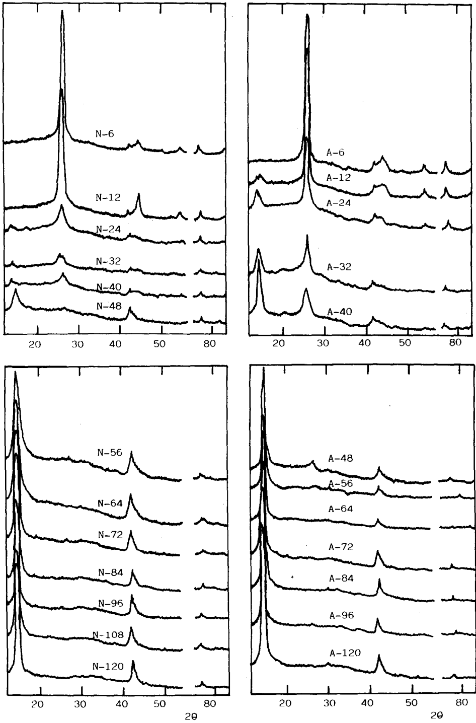
Fig. 1. Powder diagrams of the graphite oxidation products.
