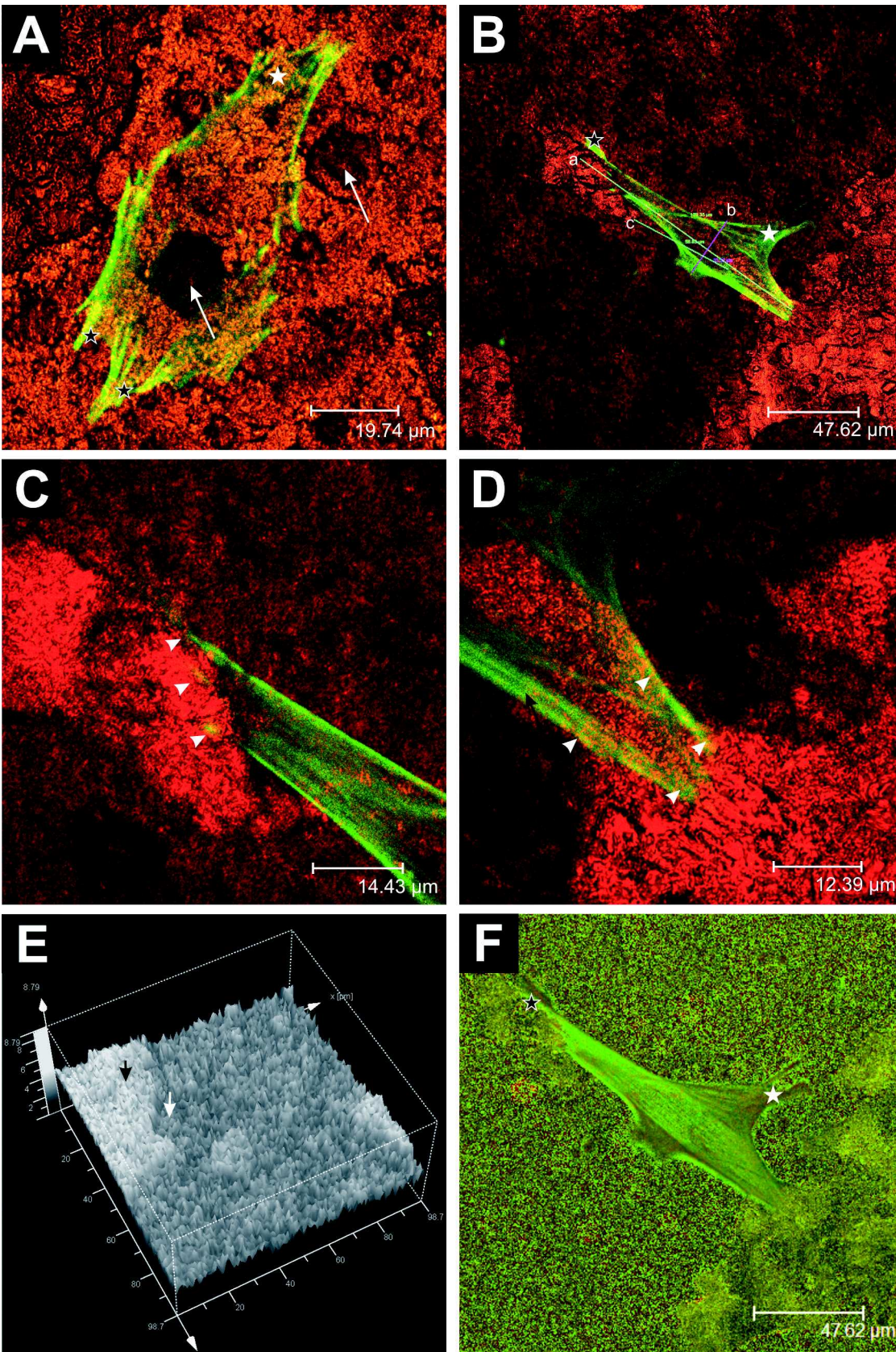
Fig. 3. CLSM image combining the fluorescence and reflection modes to illustrate cell-disk interaction in a TiCP Osseotite® disk. A. TiCP Osseotite® disks (in red) showed a marked increase in the surface roughness with prominent peaks and caves (white arrow). In this case, the cell (green) appeared to be adapted to a relatively regular surface, which allowed spreading by means of the emission of wide lamellipodia (white star) and also dendritic filopodia (black star). x 63.0, Zoom 2.41. In contrast, in B , the surface presented deeper valleys and more randomly distributed peaks than is the case for A . The cells, thus, presented an increasingly polarised spreading with emission of either wide lamellipodia (white star) or long filopodia (black star). Marked with a, b the main axis of the cell that determined the axial ratio around 3.5. Marked with c, the representative distance between peaks, as described in the text. x 63.0, Zoom 2.41. In C , with a zoom of 3.30, the focal adhesion sites, in yellow, in the apical part of the cell determined by contact of the actin stress fibers with the surface peaks are marked with white arrowheads. x 63.0. D shows at higher magnification, the yellow basal focal contacts (arrowhead) established between stress fibers (black arrow) and surface peaks. x 63.0, zoom 3.84. E. Topographical (3D) profilometric image of TiCP Osseotite® surface by confocal microscopy. Peaks, black arrow, valleys, white arrow. F. Topographical (2D) reconstruction of a 3D series obtained with the CLSM, showing the distribution of stress fibers (green), mainly in the filopodia (black star) and lamellipodia (white star), that are oriented to the focal adhesion sites in a NHOst cell growing on the rough Osseotite® surface (mixed red). Peaks, black arrow, valleys, white arrow. x 63. Zoom 1.
