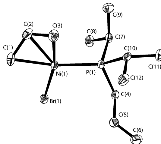
Fig. 2 ORTEP drawing (50% thermal ellipsoids) of the complex [\text{Ni}(\eta^3\text{-CH}_2\text{CHCH}_2)\text{Br}(\kappa^1 P\text{-P}^i\text{Pr}_2\text{CH}_2\text{CH}=\text{CH}_2)] ( 2 ). Selected bond lengths (Å) and angles (°) with estimated standard deviations in parentheses: Ni(1)–C(1) 2.057(4); Ni(1)–C(2) 1.998(4); Ni(1)–C(3) 1.998(4); Ni(1)–P(1) 2.1924(11); Ni(1)–Br(1) 2.3324(8); C(1)–C(2) 1.386(5); C(2)–C(3) 1.389(6); C(4)–C(5) 1.496(5); C(5)–C(6) 1.321(5); Br(1)–Ni(1)–P(1) 99.11(3); C(1)–C(2)–C(3) 118.8(4).
