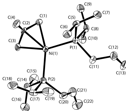
Fig. 3 ORTEP drawing (50% thermal ellipsoids) of the complex cation [\text{Ni}(\eta^3\text{-CH}_2\text{C}(\text{CH}_3)\text{CH}_2)(\kappa^1 P\text{-P}^i\text{Pr}_2\text{CH}_2\text{CH}=\text{CH}_2)_2]^+ in 5b . Hydrogen atoms have been omitted. Selected bond lengths (Å) and angles (°) with estimated standard deviations in parentheses: Ni(1)–C(1) 2.049(4); Ni(1)–C(2) 2.040(4); Ni(1)–C(3) 2.047(4); Ni(1)–P(1) 2.2215(13); Ni(1)–P(2) 2.2386(13); C(1)–C(2) 1.399(6); C(2)–C(3) 1.396(7); C(2)–C(4) 1.499(7); C(11)–C(12) 1.489(6); C(12)–C(13) 1.310(7); C(20)–C(21) 1.475(7); C(21)–C(22) 1.311(8); P(1)–Ni(1)–P(2) 110.61(5); C(1)–C(2)–C(3) 116.2(5); torsion angle C(11)–P(1)–P(2)–C(20) 21.4(2).
