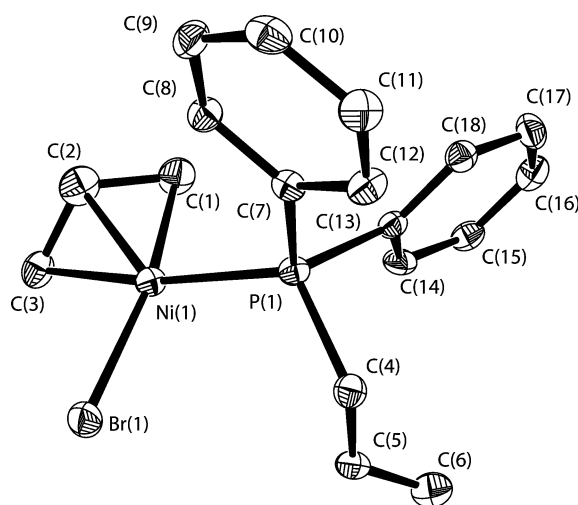
Fig. 1 ORTEP drawing (50% thermal ellipsoids) of the complex [\text{Ni}(\eta^3\text{-CH}_2\text{CHCH}_2)\text{Br}(\kappa^1 P\text{-PPh}_2\text{CH}_2\text{CH}=\text{CH}_2)] ( 1 ). Selected bond lengths (Å) and angles (°) with estimated standard deviations in parentheses: Ni(1)–C(1) 1.999(3); Ni(1)–C(2) 1.999(3); Ni(1)–C(3) 2.066(3); Ni(1)–P(1) 2.1941(10); Ni(1)–Br(1) 2.3224(7); C(1)–C(2) 1.415(5); C(2)–C(3) 1.366(5); C(4)–C(5) 1.489(4); C(5)–C(6) 1.313(5); Br(1)–Ni(1)–P(1) 97.77(2); C(1)–C(2)–C(3) 120.4(3).
