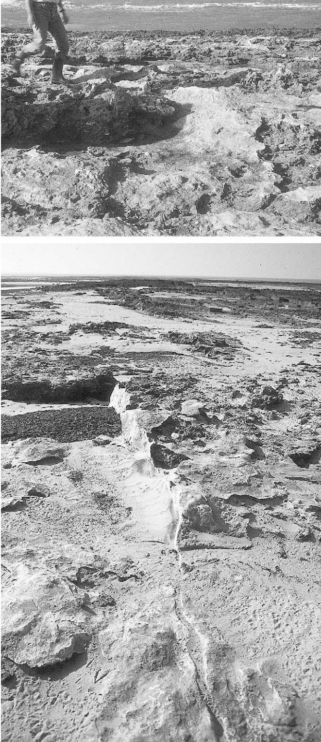
Fig. 7. Late Pleistocene (MIS 3) beach deposit forming a wide shore platform at Torregorda. A laminated calcareous crust can be seen covering most part of the beach deposit.
