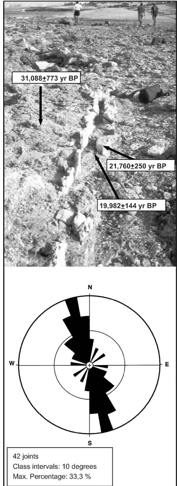
Fig. 8. Open fractures on Upper Pleistocene beach deposit at Torregorda (see Fig. 3 for location). A white calcrete can be seen filling the fracture, where two samples were taken for radiometric dating. Below: Rose of fractures and joints measured in the zone.
